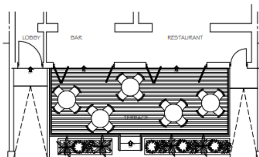
PARTIAL GROUND FLOOR PLAN
